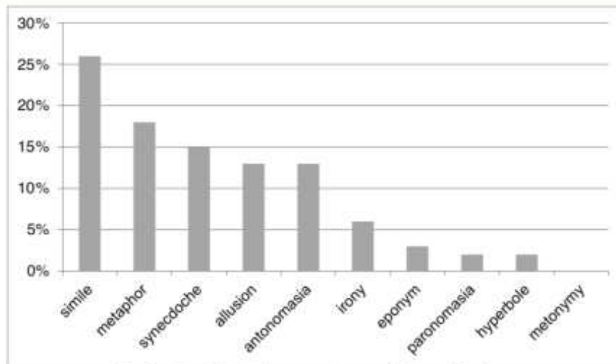
Fig. 2. The Chart of percentage of Figurative Language
